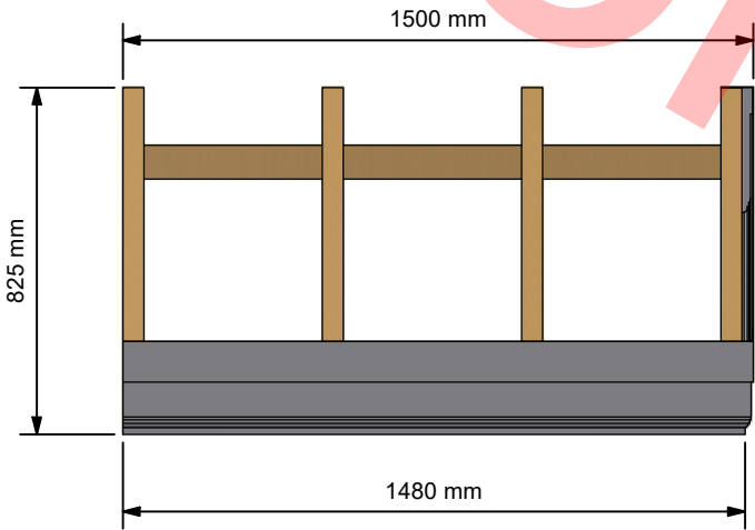
Front Elevation ( 1 : 20 )
