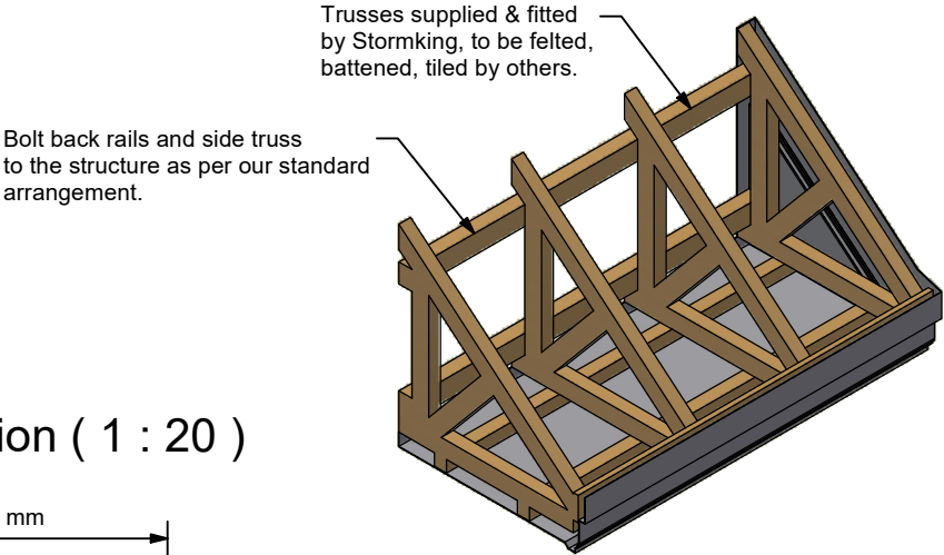
Auxiliary View ( 1 : 25 )
