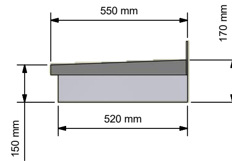
Side Elevation
