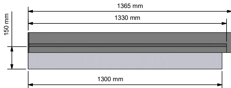
Front Elevation ( 1 : 15 )
