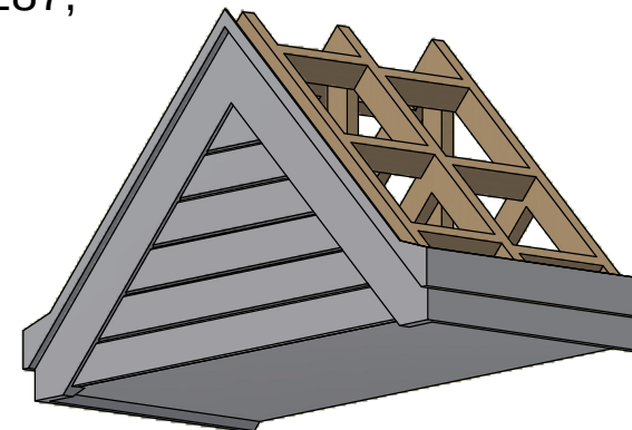
Auxiliary View ( 1:20 )
