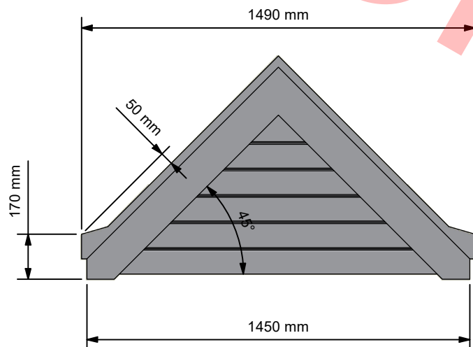
Front Elevation ( 1:20 )
