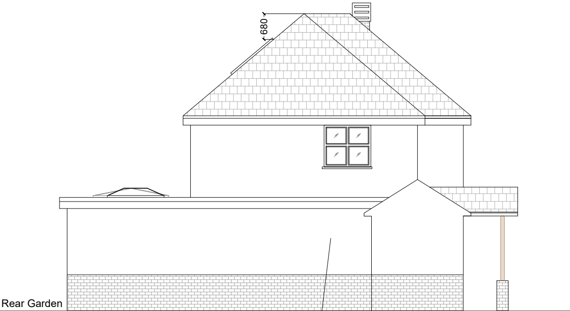
Proposed East Elevation 1:100 @A3
