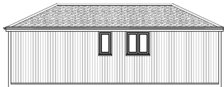
ELEVATION C
