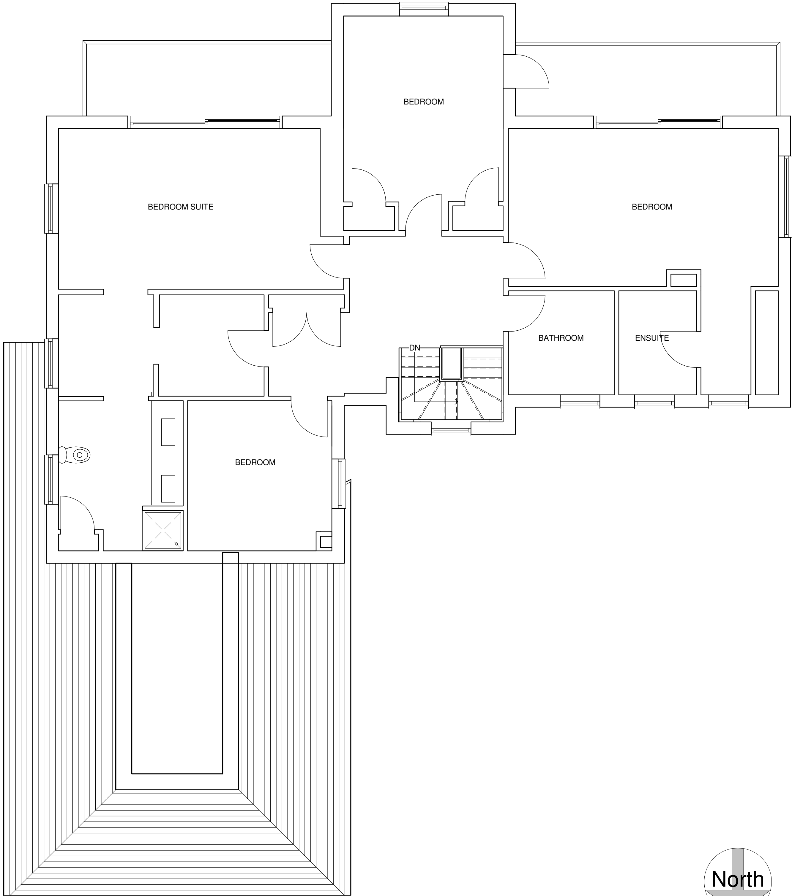
2 1 - Existing First Floor 1 : 50
