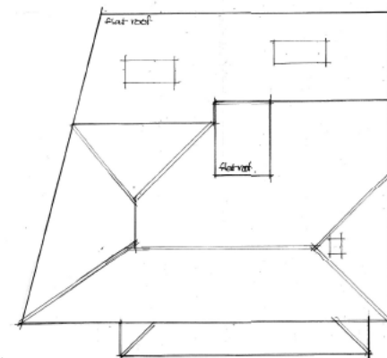
roof plan 1:100
