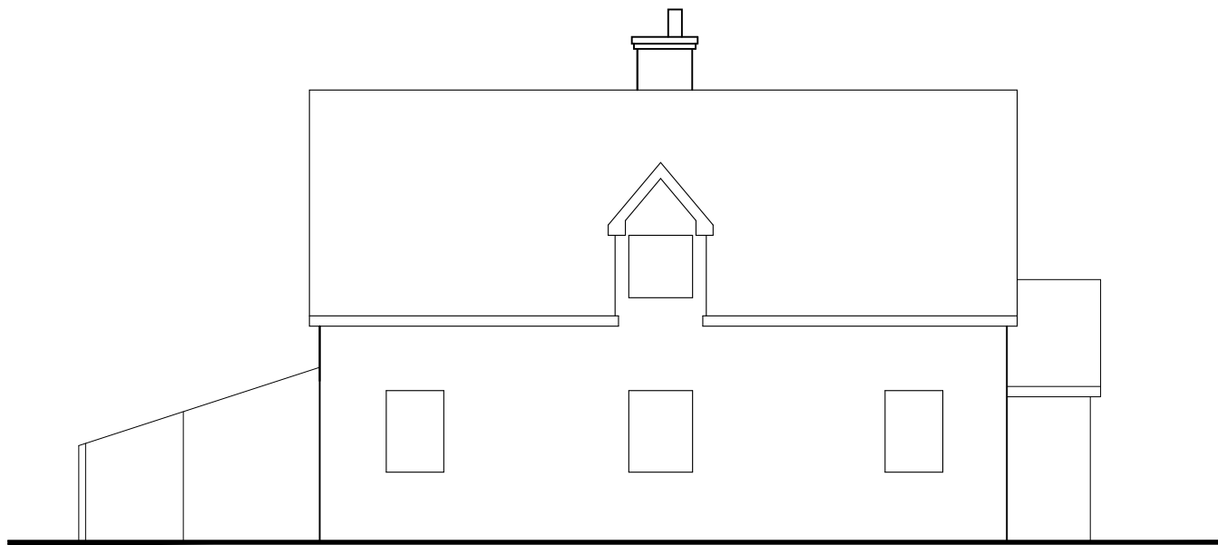
WEST ELEVATION 1:100
