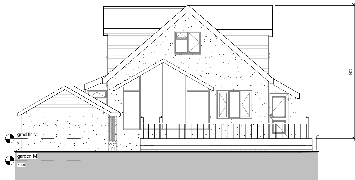
Existing Elevation-Rear
