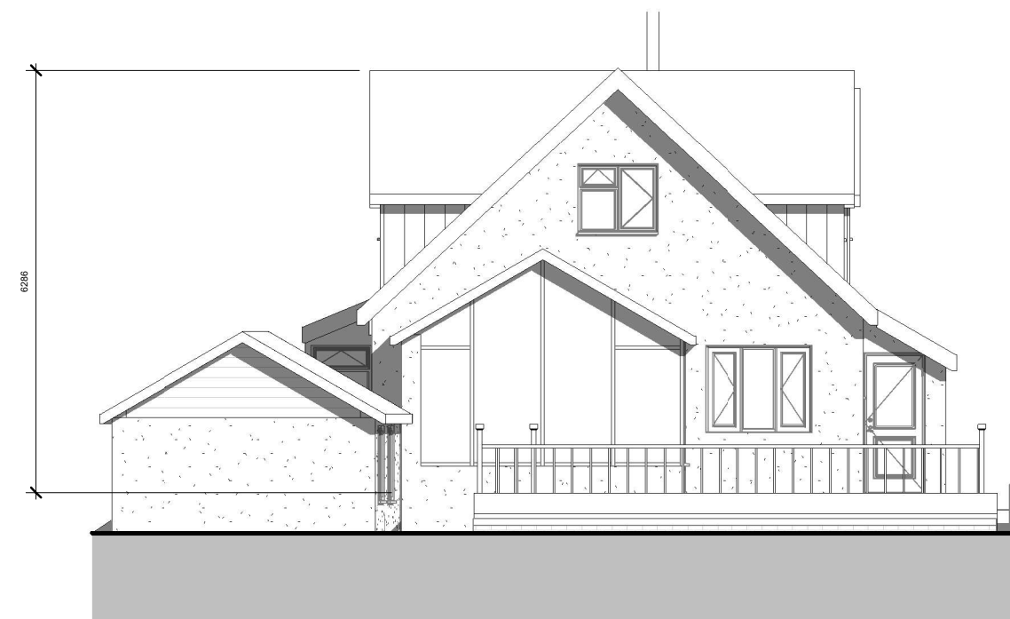
Proposed Elevation-Rear
