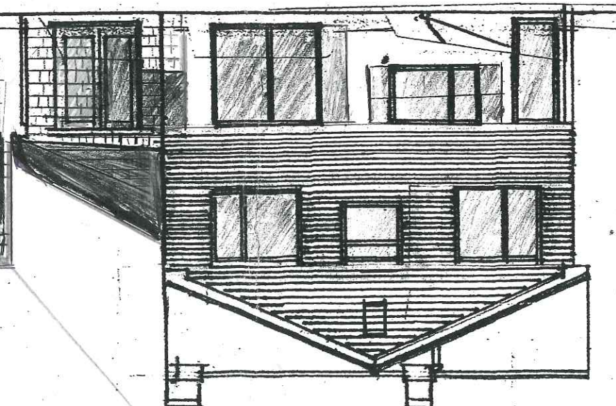
PROPOSED ELEVATION
