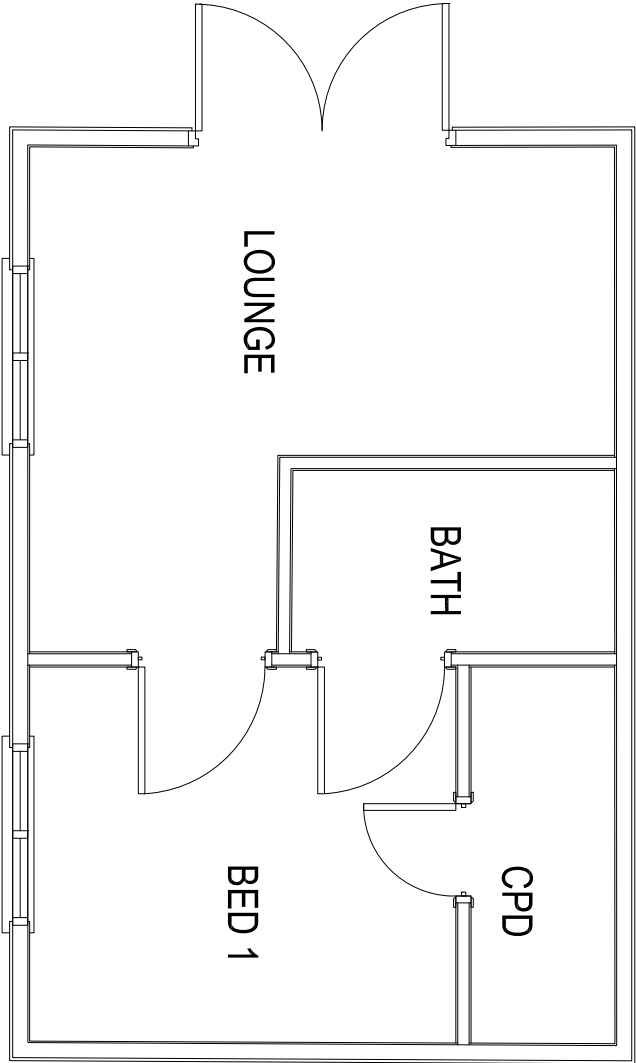
FLOOR PLAN
