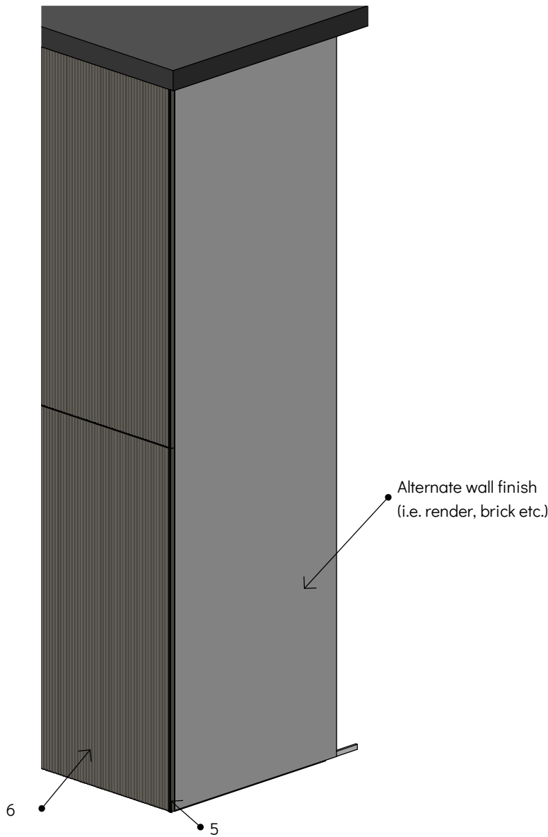
Iso: Cladding Corner Detail - showing interface of vertical Panel cladding with a render or brick wall finish 1:50
