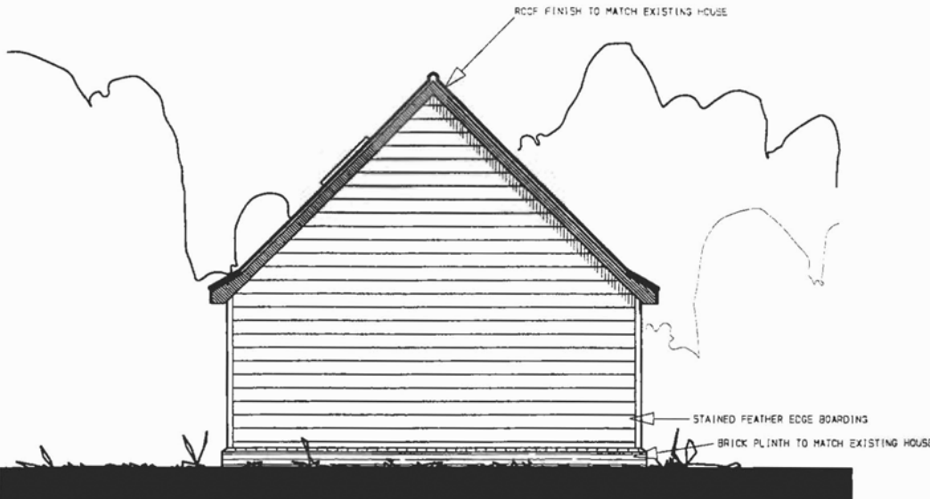
SIDE ELEVATION
