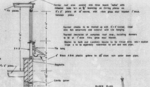
SECTION THRU REAR DORMER
