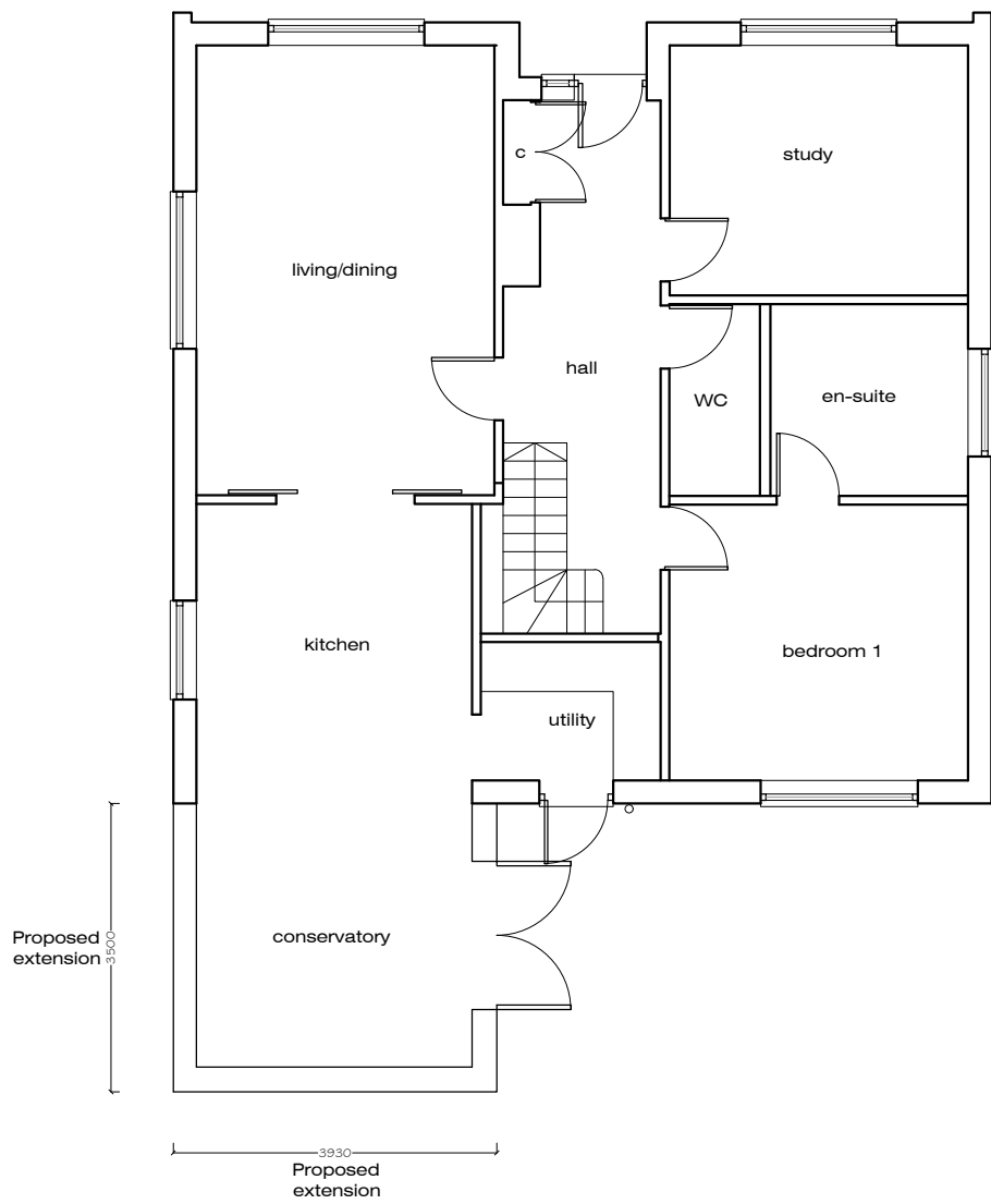
Ground Floor Plan - As Proposed
