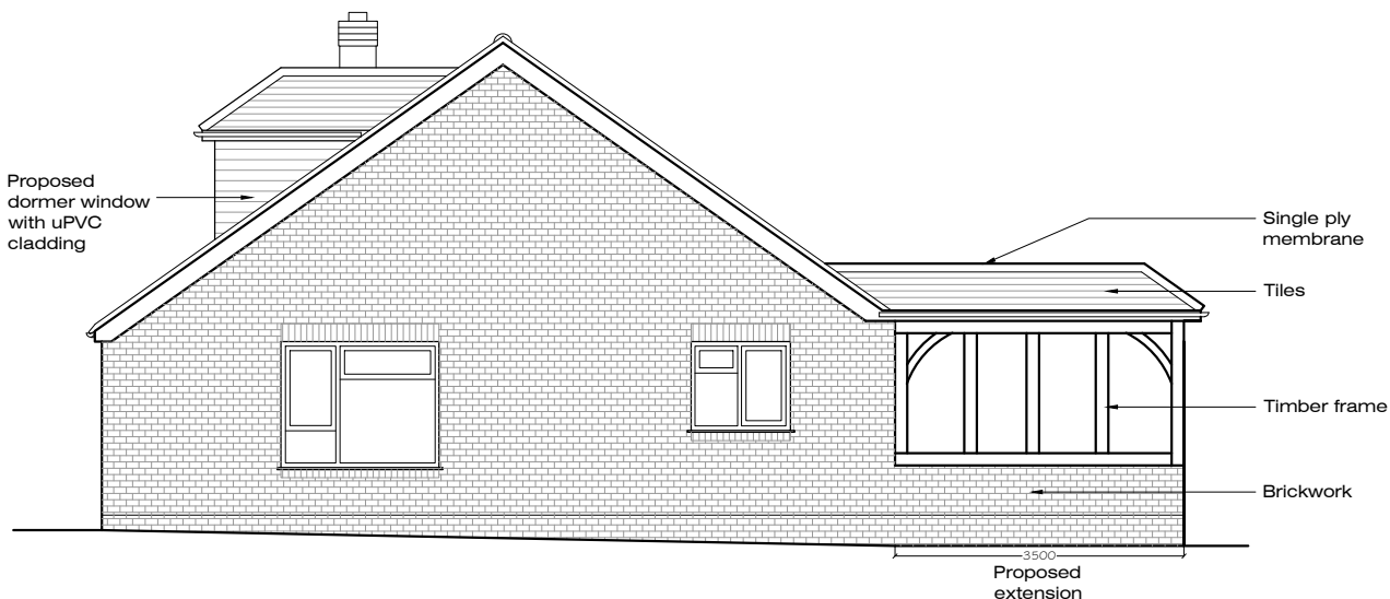
North-East (Side) Elevation - As Proposed
