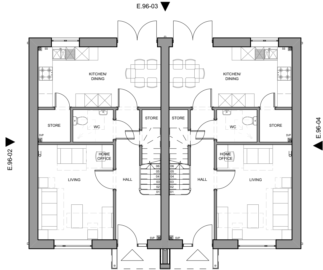
GF-Ground Floor
