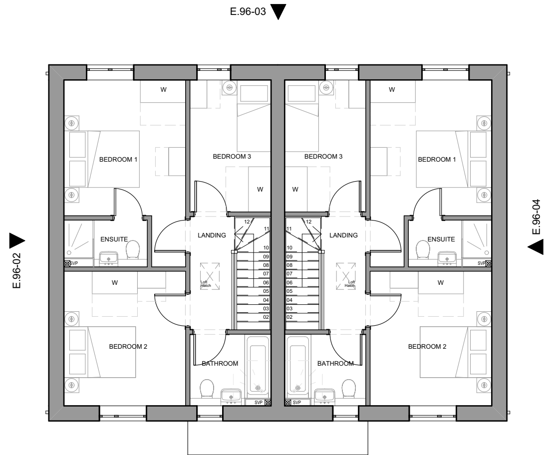
01-First Floor
