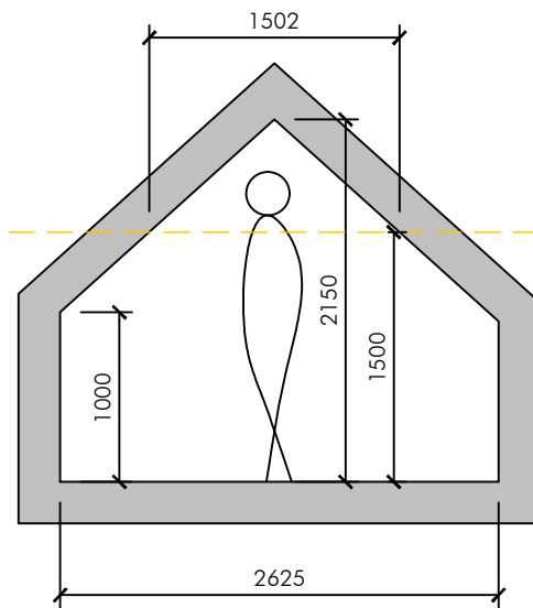
Section through study Scale 1:50
