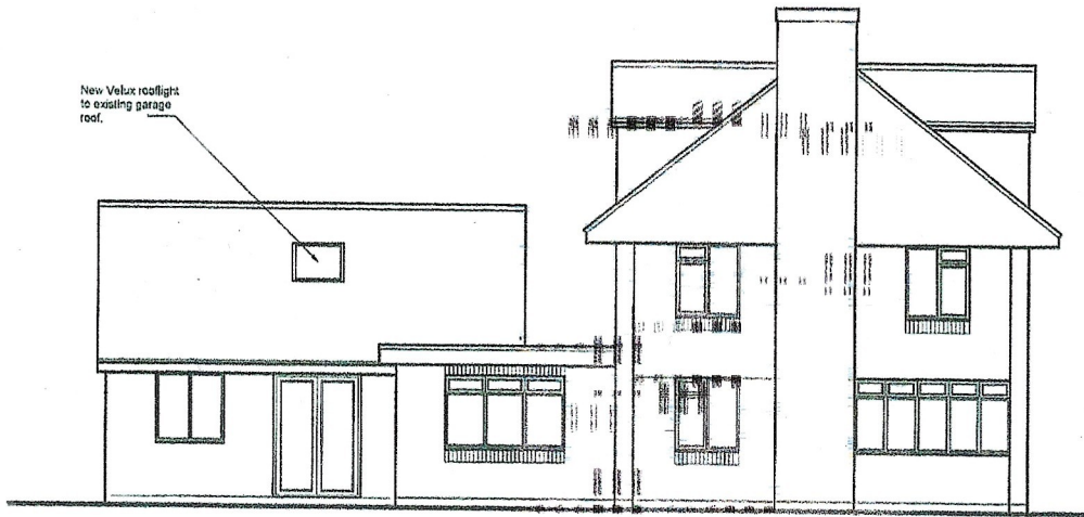
PROPOSED WEST ELEVATION 1:50
