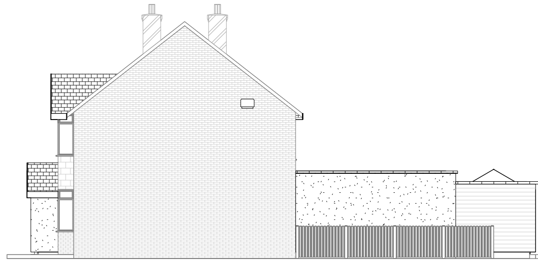
Proposed Elevation-Right side
