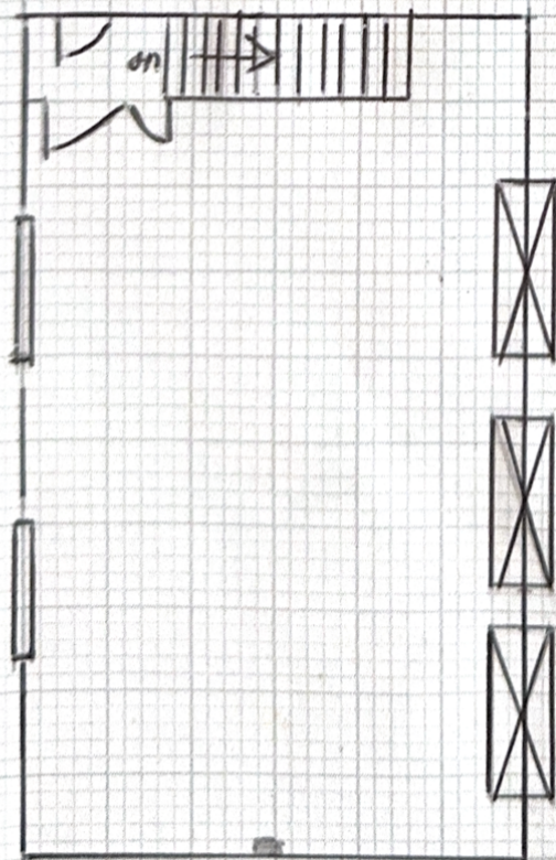
GROUND FLOOR PLAN AS EXISTING
