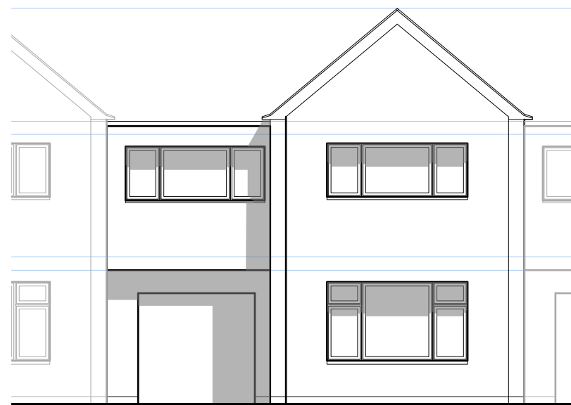
5 West Elevation (Existing) Scale: 1:100
