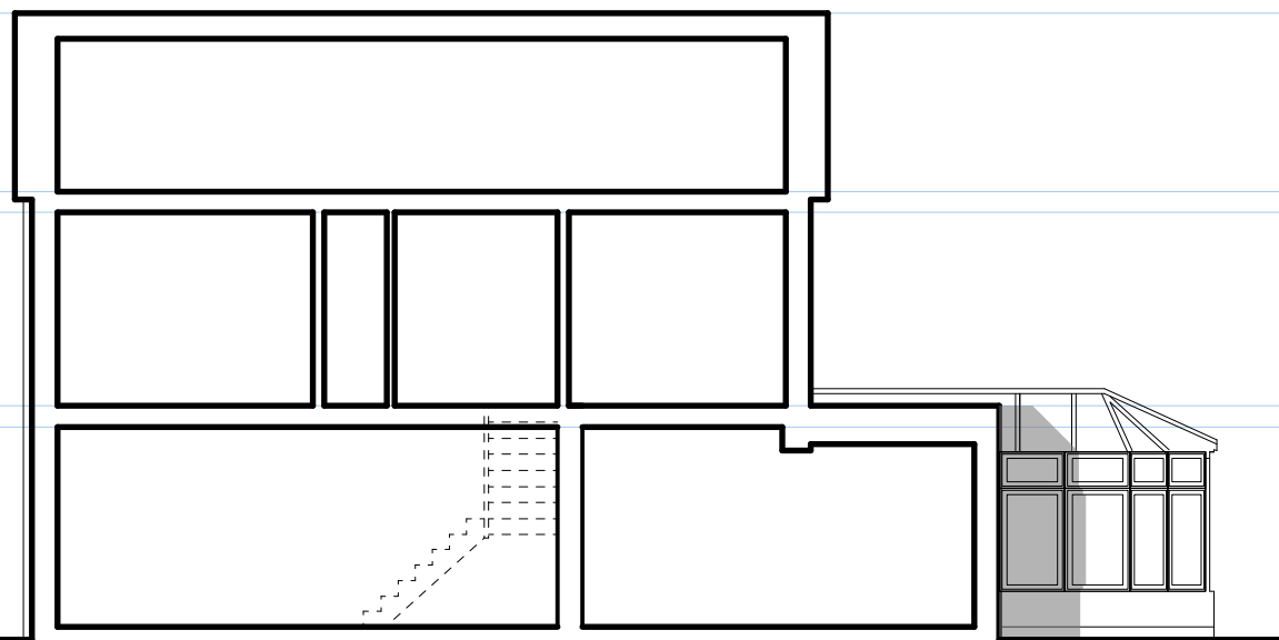
4 South Elevation (Existing) Scale: 1:100
