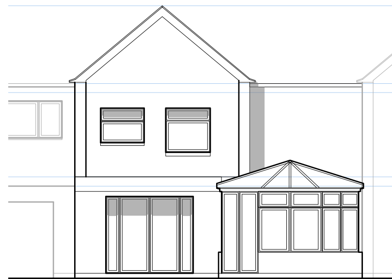
6 East Elevation (Existing) Scale: 1:100
