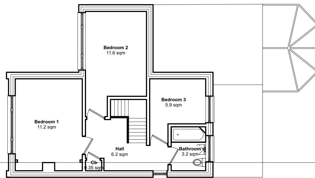
2 First Floor Plan (Existing) Scale: 1:100
