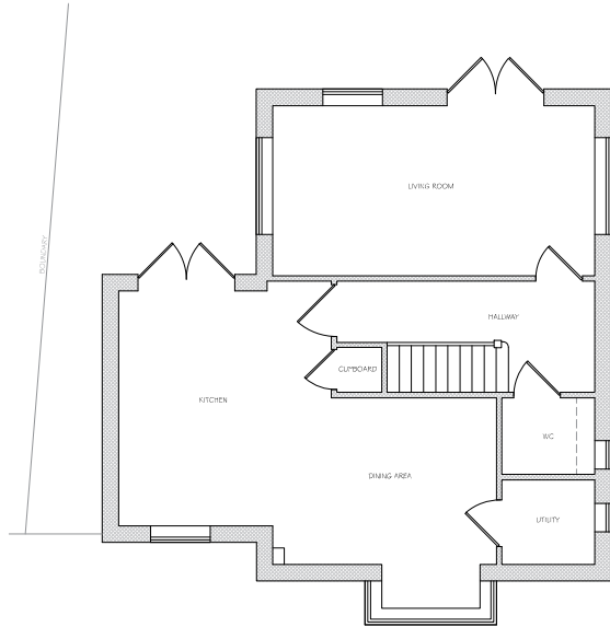
Existing Ground Floor Plan 1:100 @ A3
