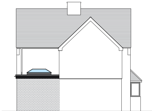
Proposed Side Elevation 1:100 @ A3
