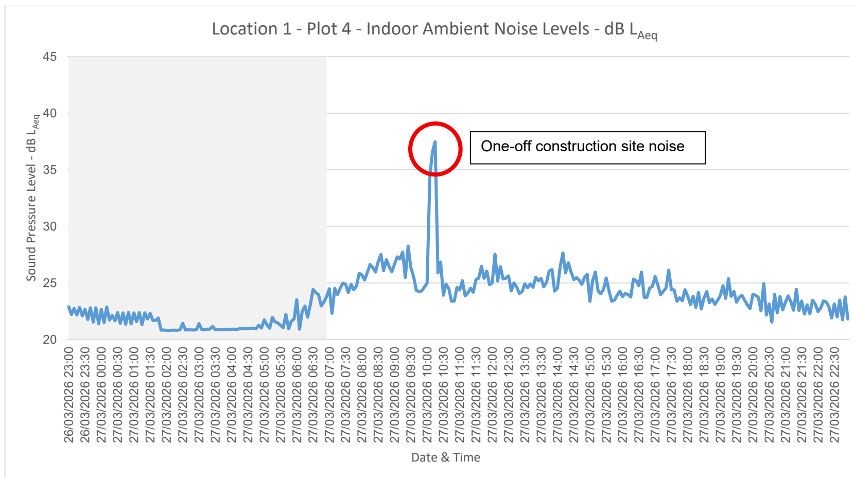
Graph 1: Location 1 – Plot 4 – L_{Aeq, 5mins} (Daytime & Night-time)
