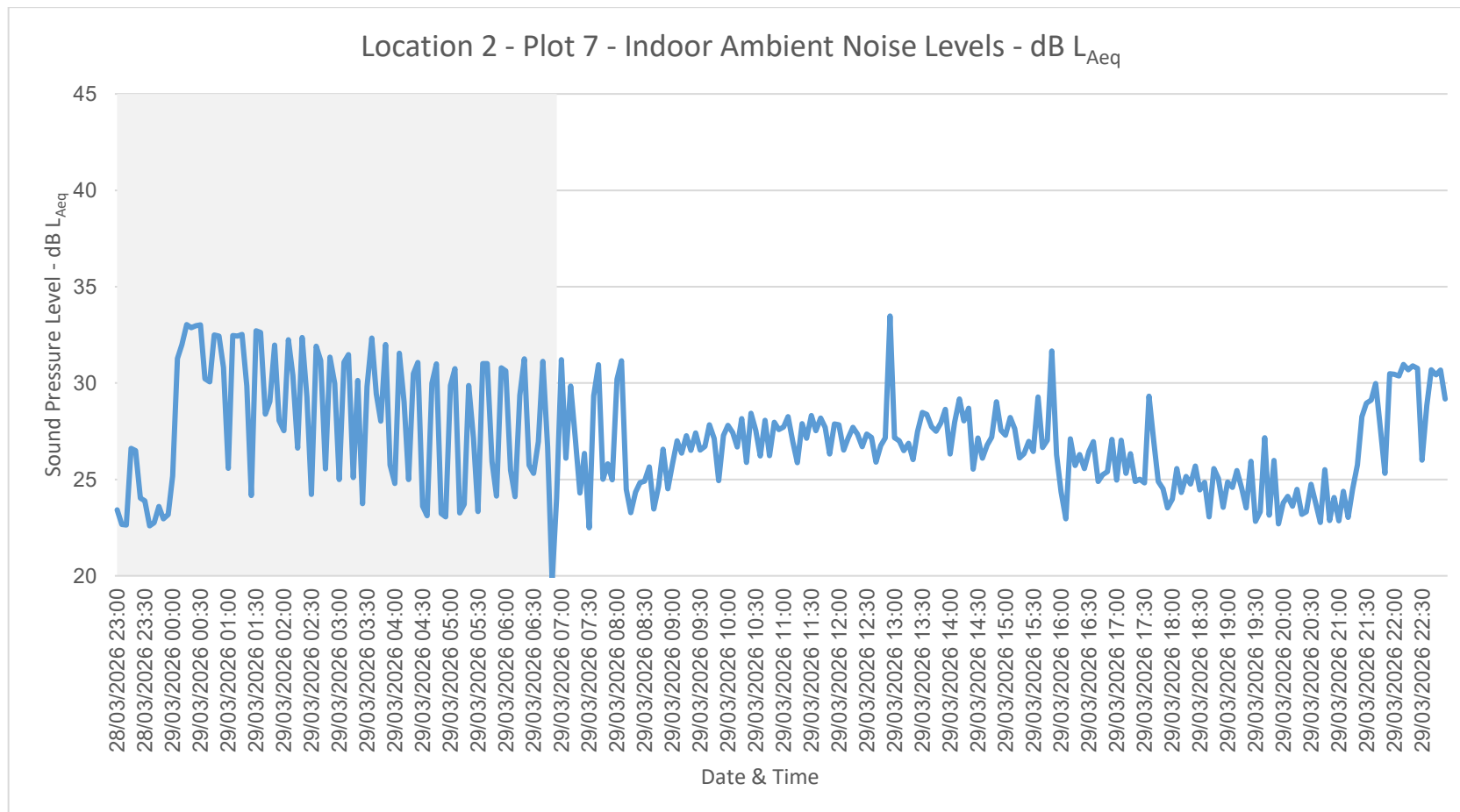
Graph 1: Location 2 – Plot 7 – L_{Aeq, 5mins} (Daytime & Night-time)
