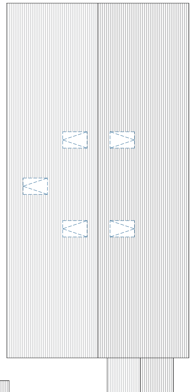
Proposed Roof Plan 1:100 @ A3
