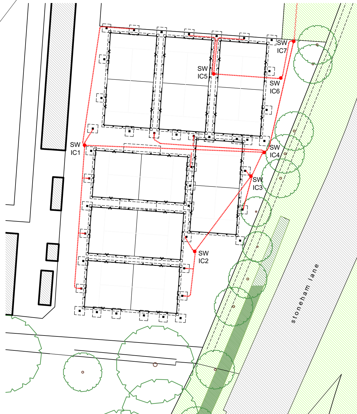
surface water drainage as proposed -1:500
