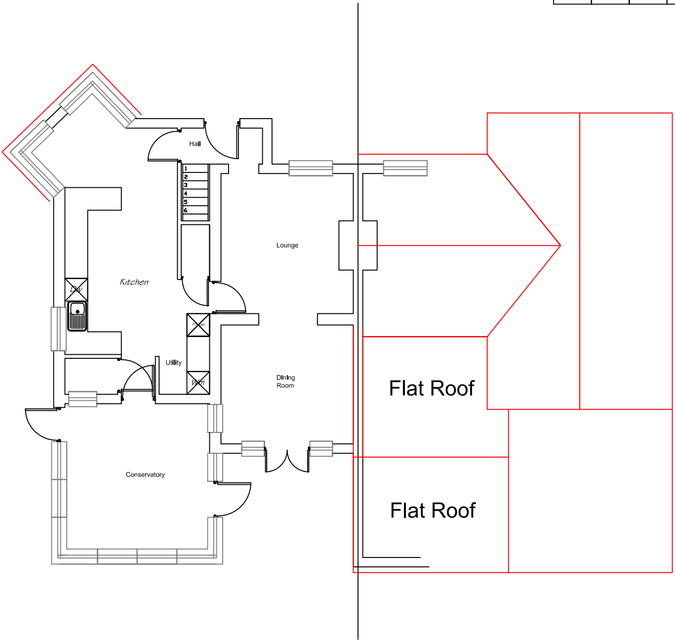
EXISTING GROUND FLOOR
