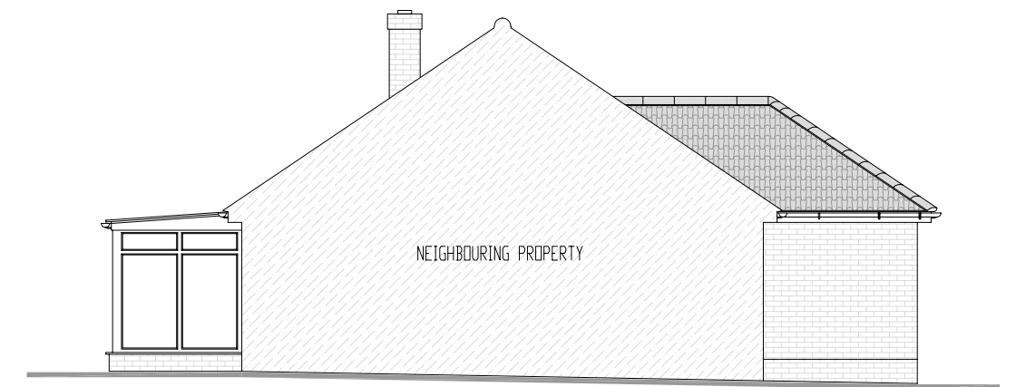
SIDE (NORTH) ELEVATION
