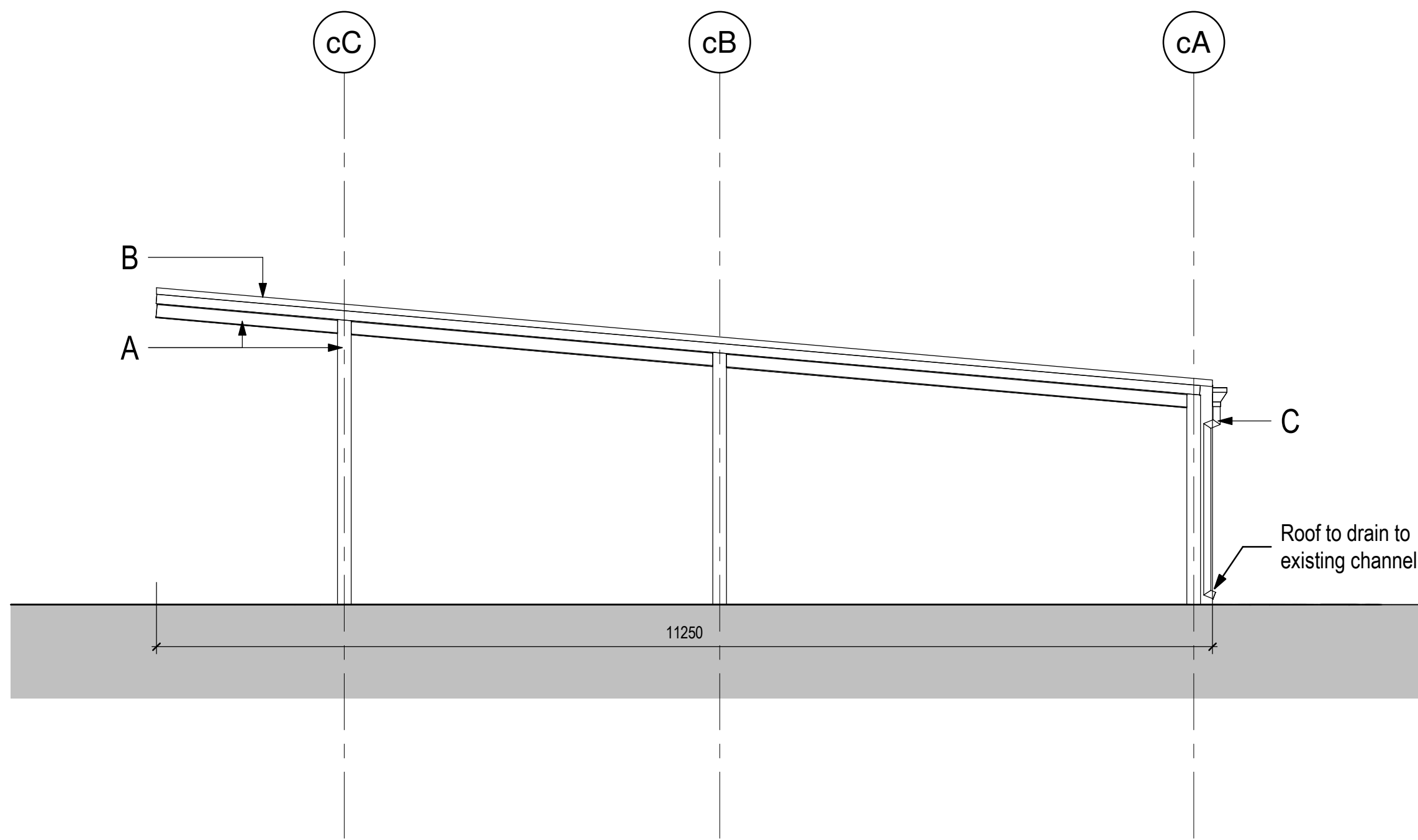
1| Canopy Elevation 1 Scale: 1 : 50
