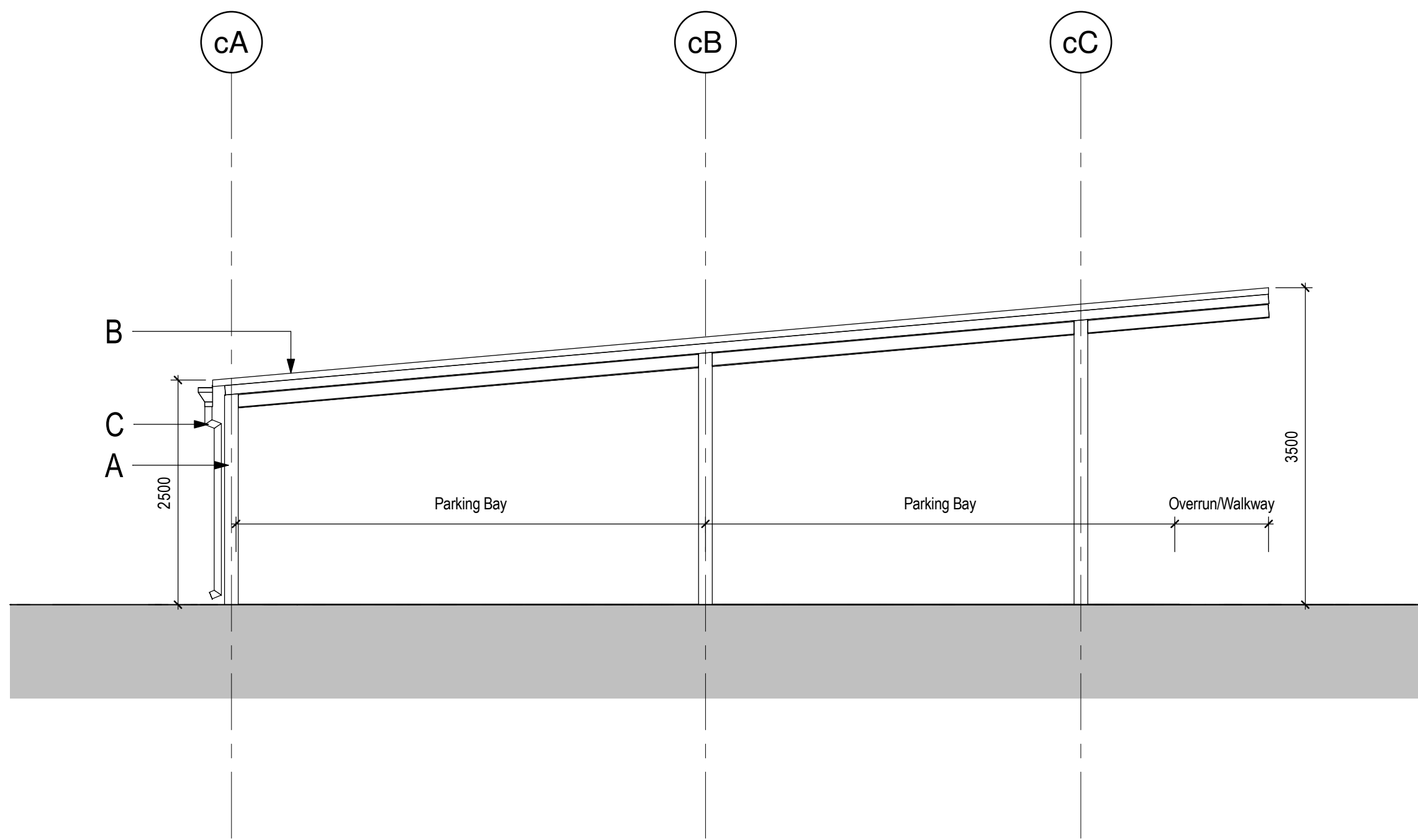
2| Canopy Elevation 2 Scale: 1 : 50
