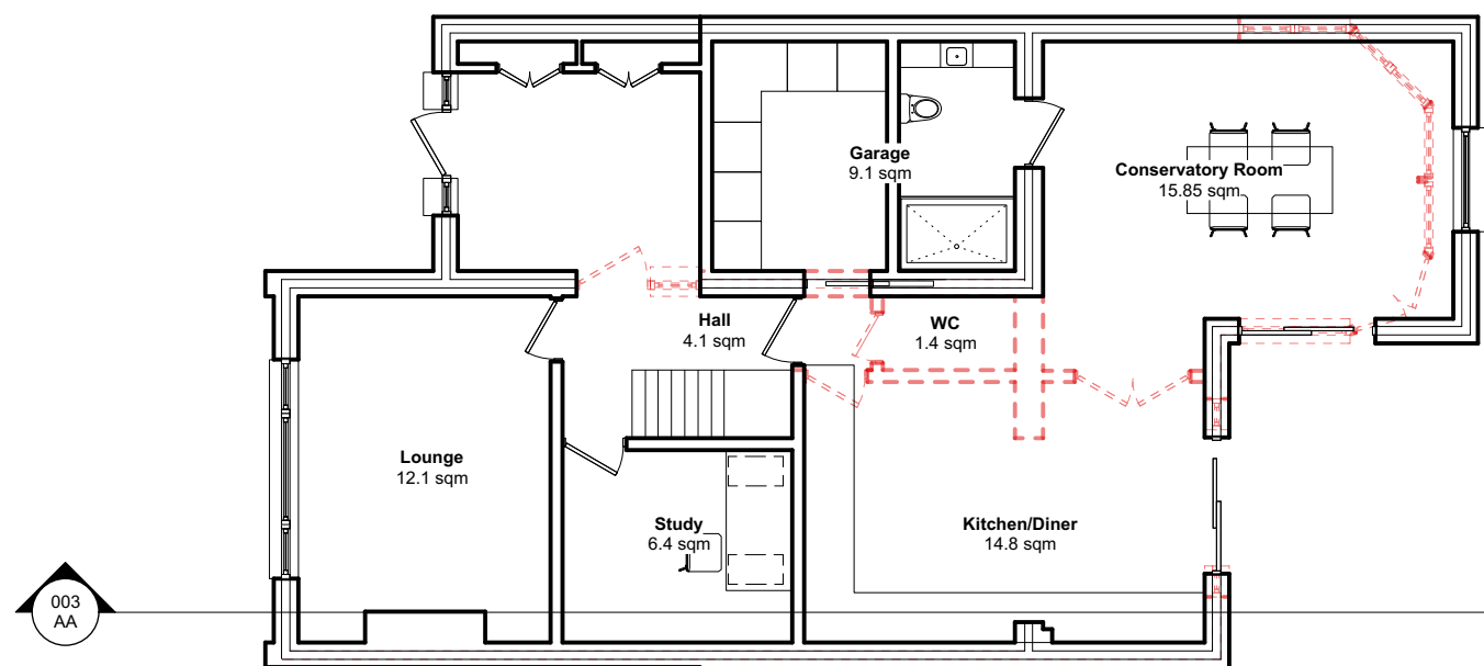
1 Ground Floor Plan (Proposed) Scale: 1:100
