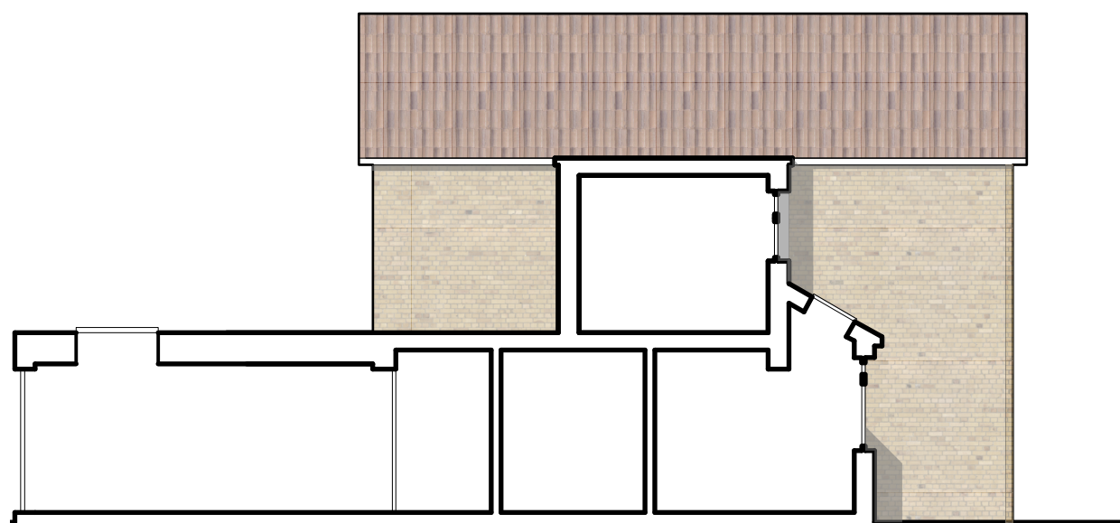
3 North Elevation (Proposed) Scale: 1:100
