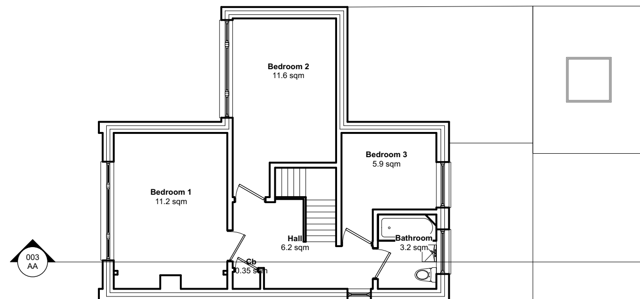
2 First Floor Plan (Proposed) Scale: 1:100
