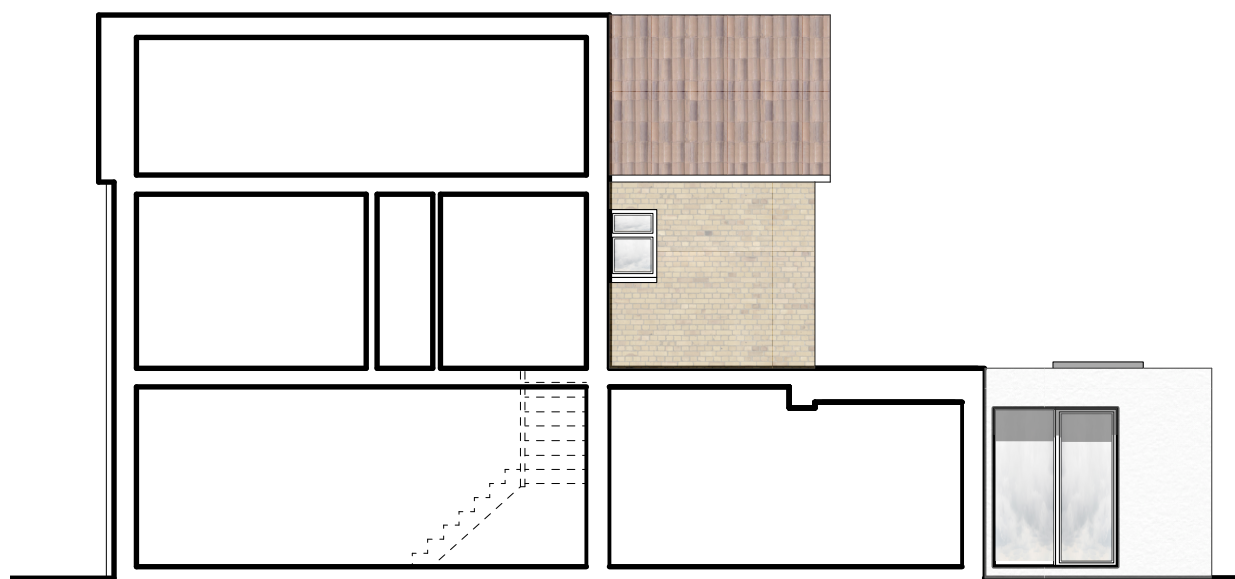
4 South Elevation (Proposed) Scale: 1:100
