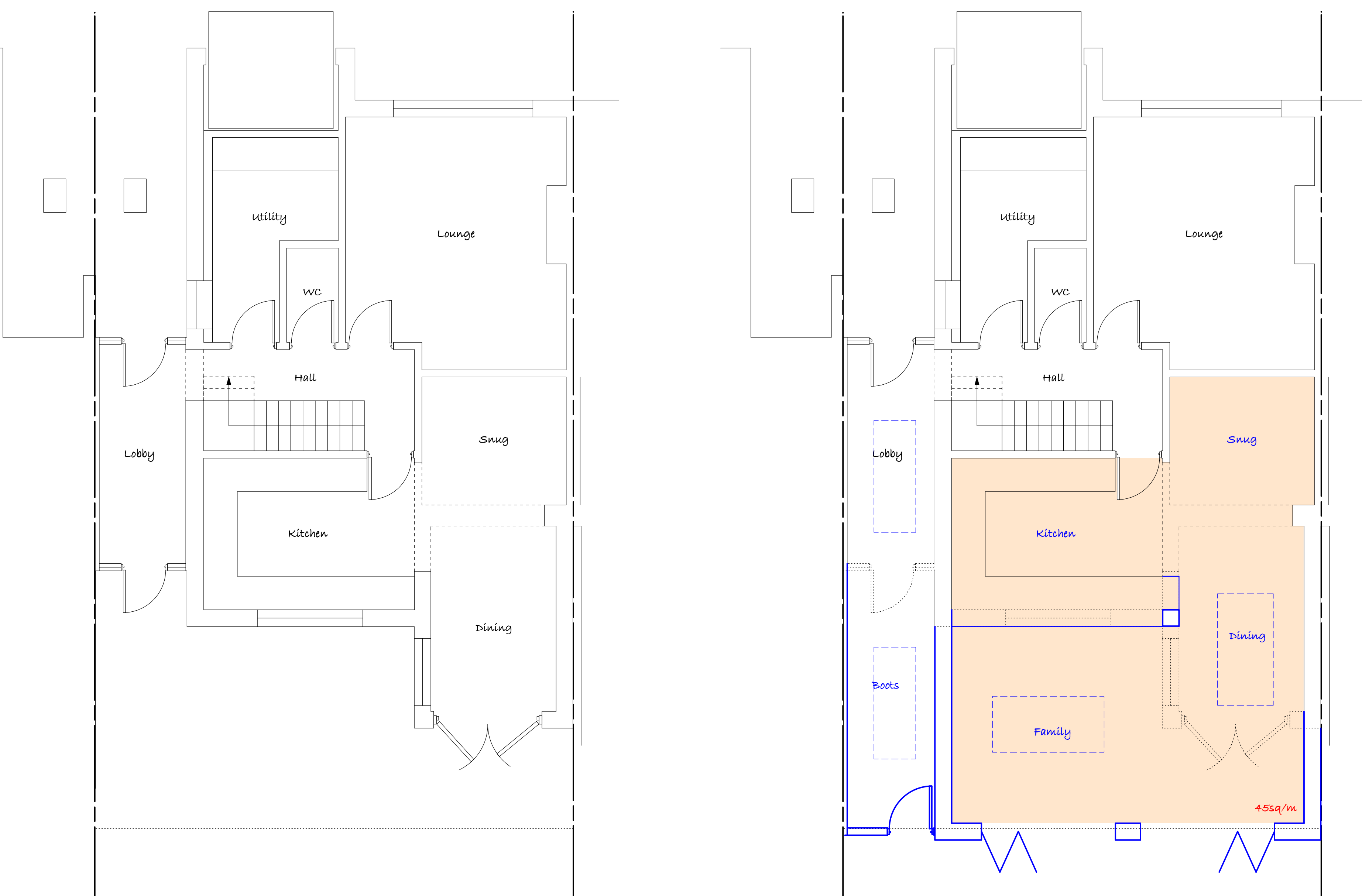
Existing Ground Floor Plan 1:50
