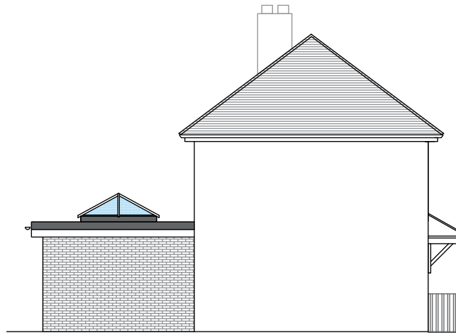
Proposed Side Elevation 1:100 @ A3
