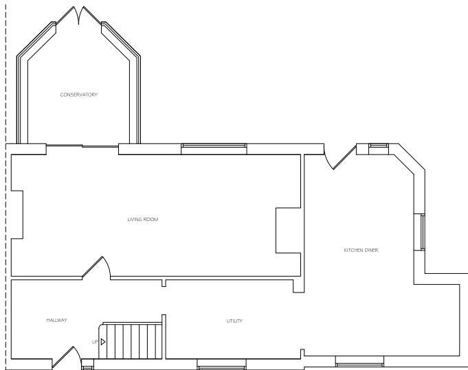
Existing Ground Floor Plan 1:100 @ A3
