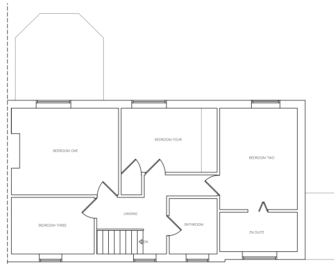
Existing First Floor Plan 1:100 @ A3
