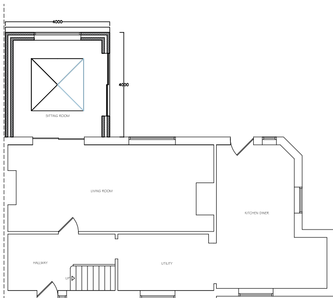
Proposed Ground Floor Plan 1:100 @ A3
