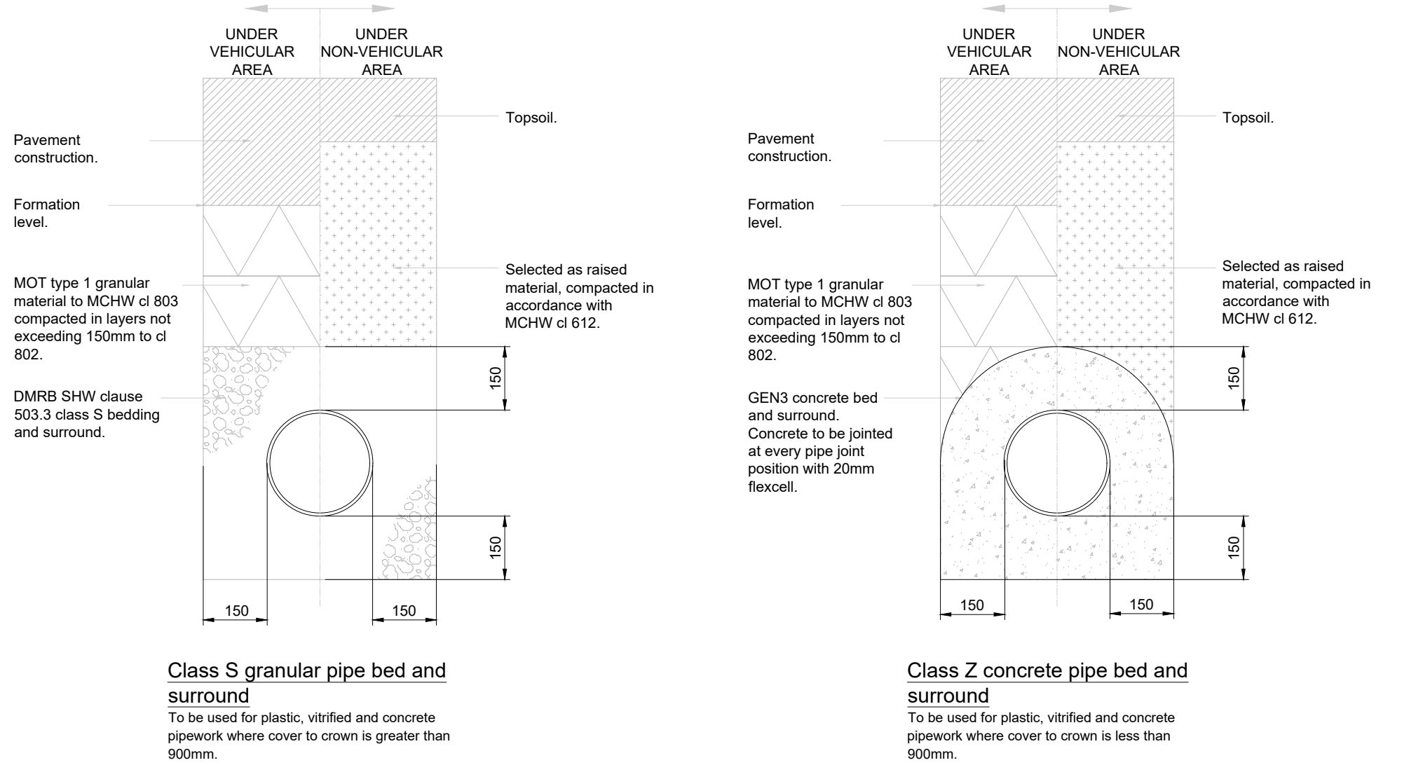
PIPE BEDDING DETAILS
