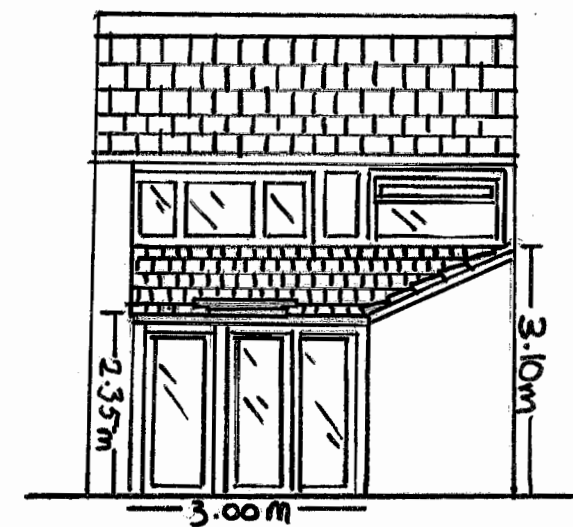
Rear Extension 1:100 Elevation
