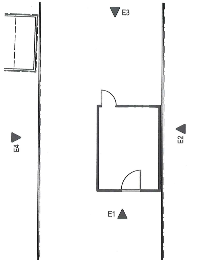
G Existing Ground Floor Plan 1:100
