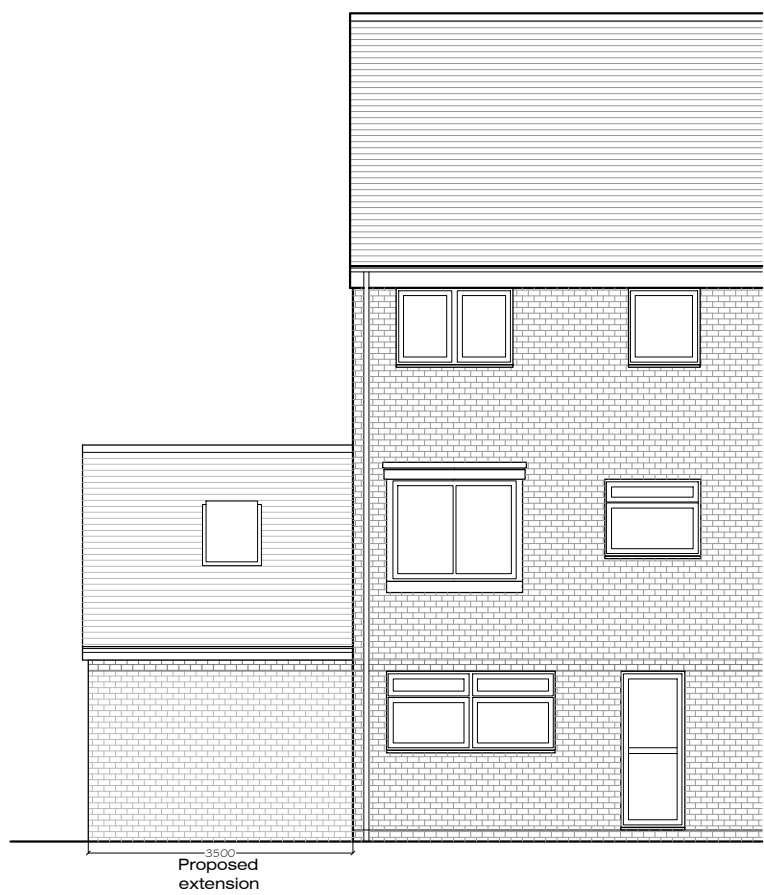
South-West (Rear) Elevation - As Proposed
