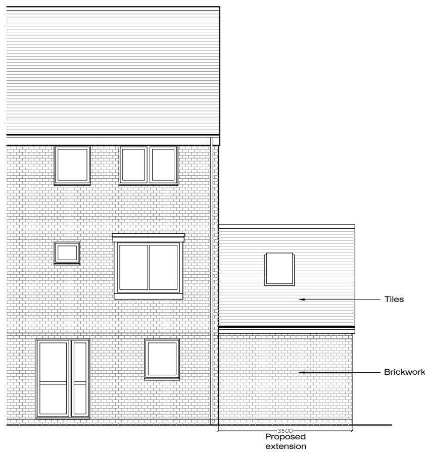
North-East (Front) Elevation - As Proposed
