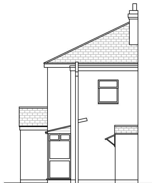
Rear Elevation
