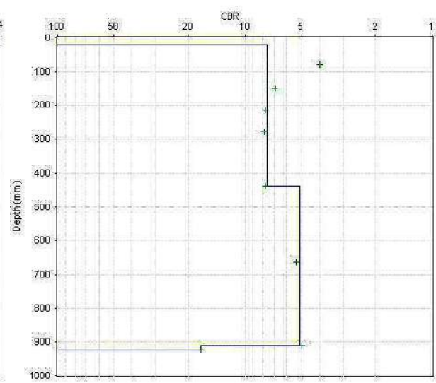
CBR Chart
