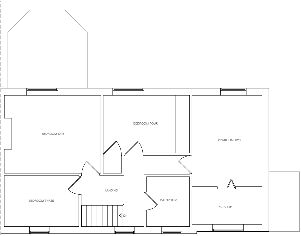
Existing First Floor Plan 1:100 @ A3
