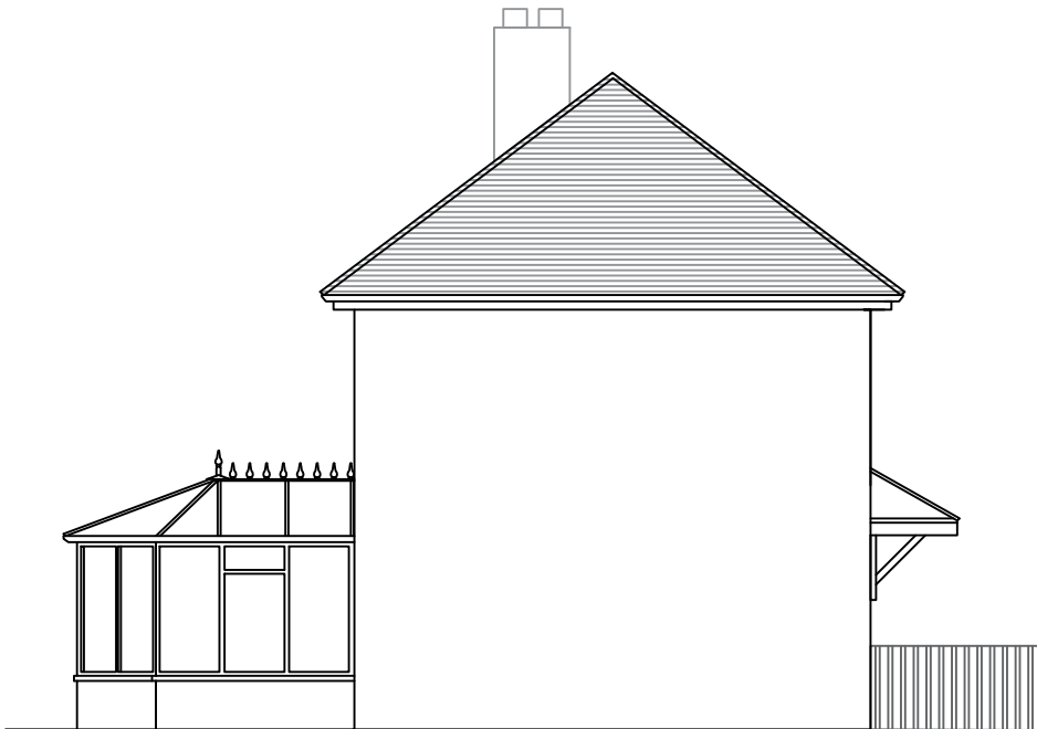
Existing Side Elevation 1:100 @ A3
