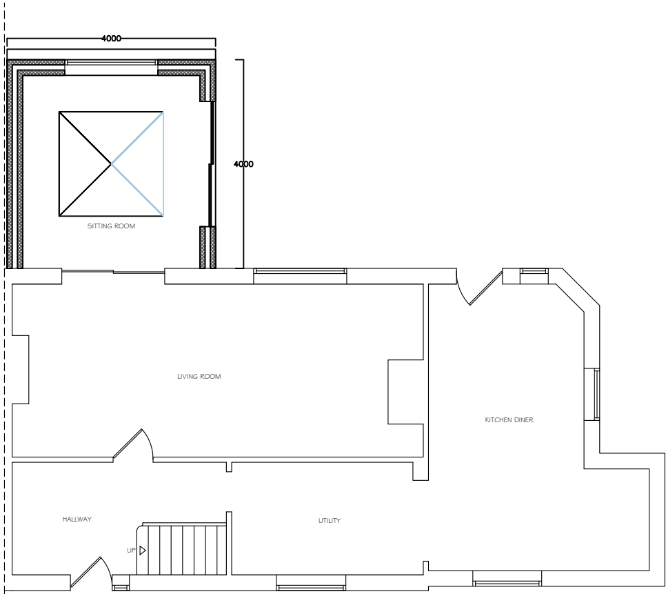
Proposed Ground Floor Plan 1:100 @ A3
