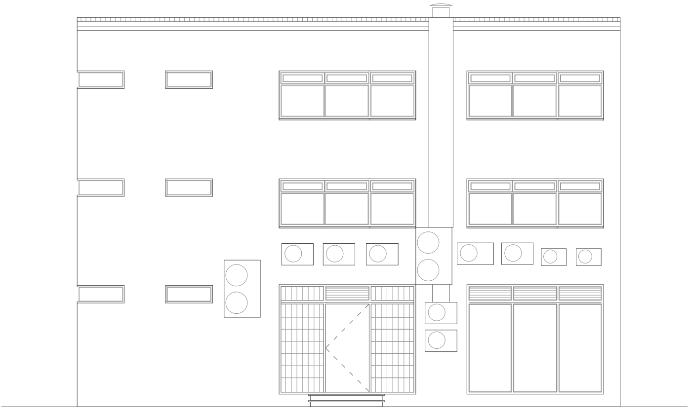
Consented Rear Elevation Scale 1 to 100 (a1)
