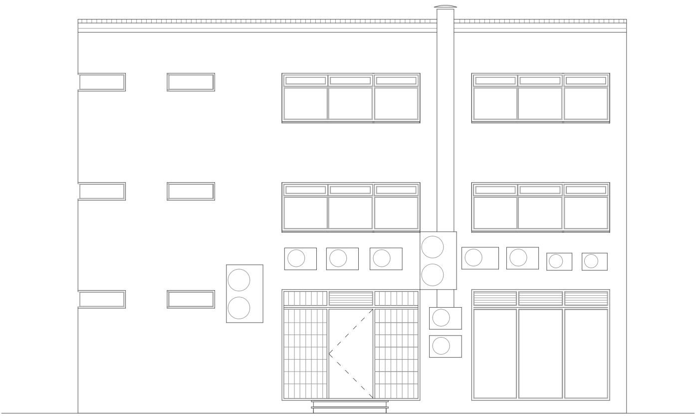
Existing Rear Elevation Scale 1 to 100 (a1)
