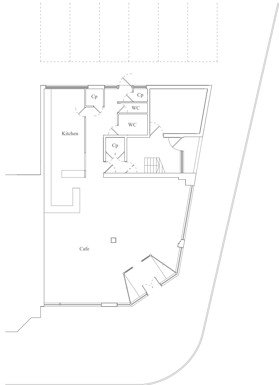
Proposed Ground Floor Scale 1 to 200 (a4)
