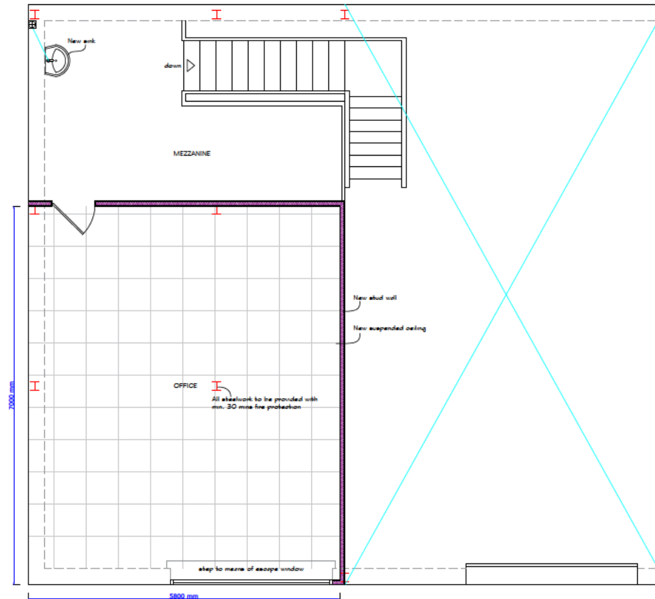
Proposed Mezzanine Floor Plan 1:100 @ A3
