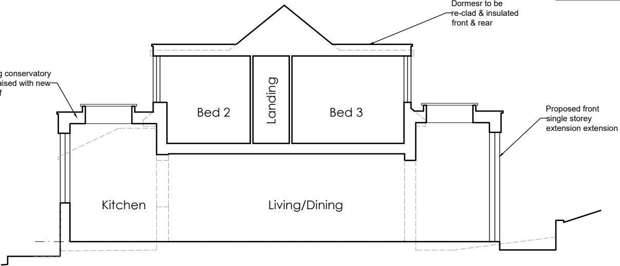
Proposed Section 1:100
