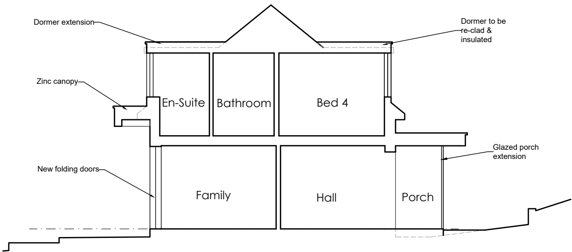
Proposed Section 1:100
