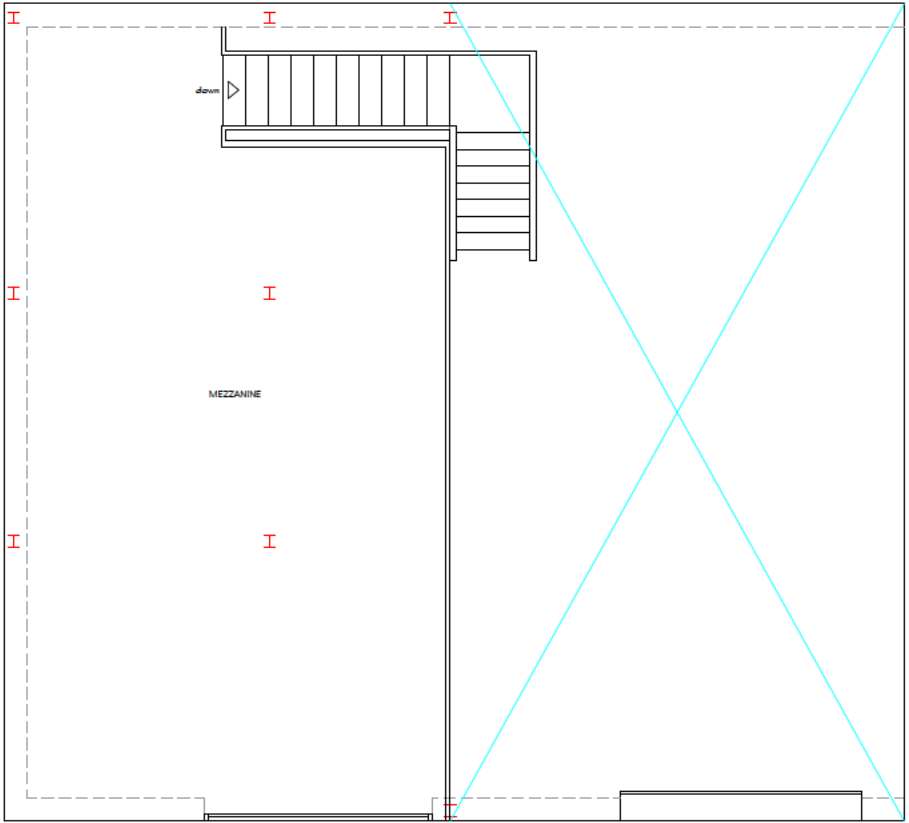
Existing Mezzanine Floor Plan 1:100 @ A3
