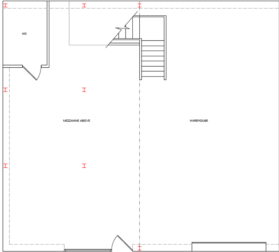
Existing Ground Floor Plan 1:100 @ A3
