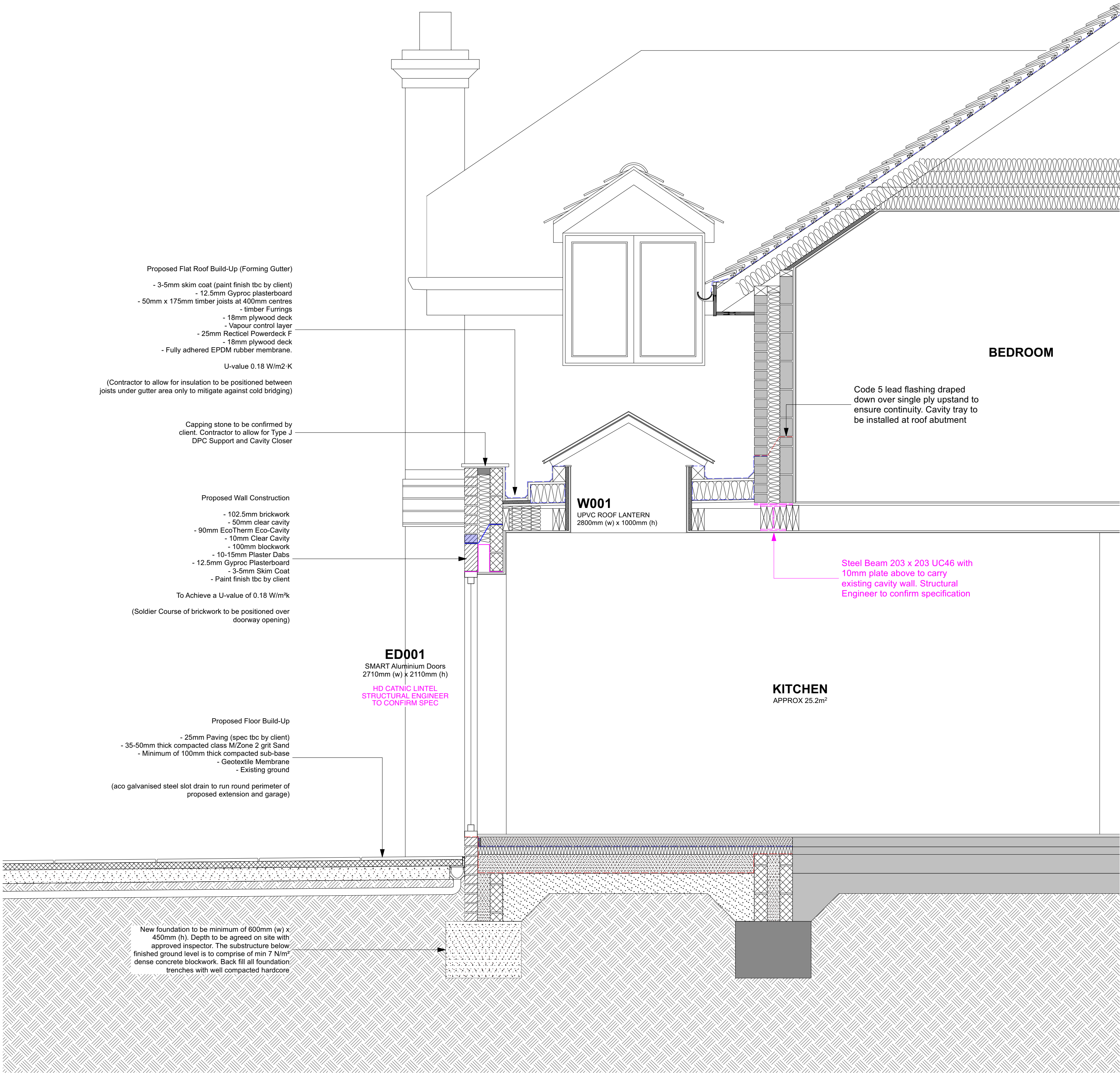
PROPOSED SECTION AA 1:20
