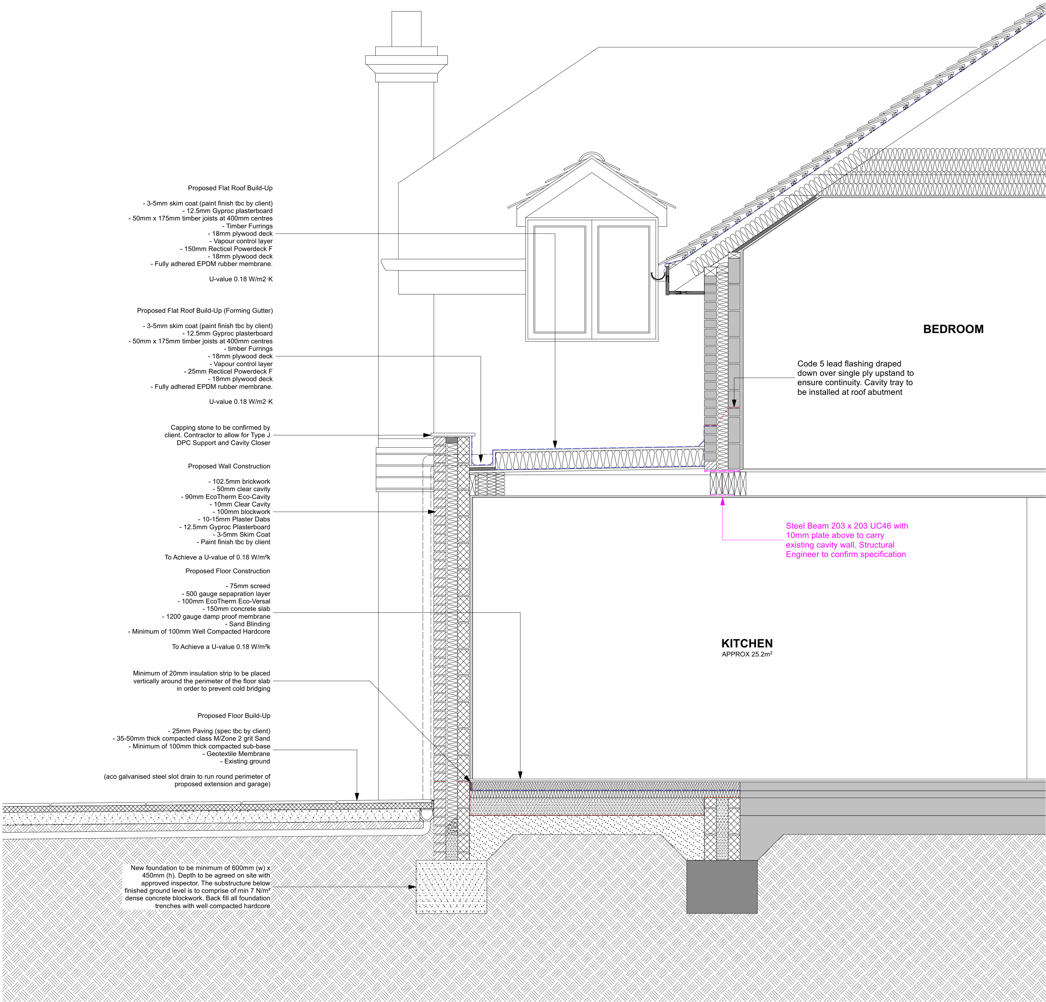
PROPOSED SECTION BB 1:20
