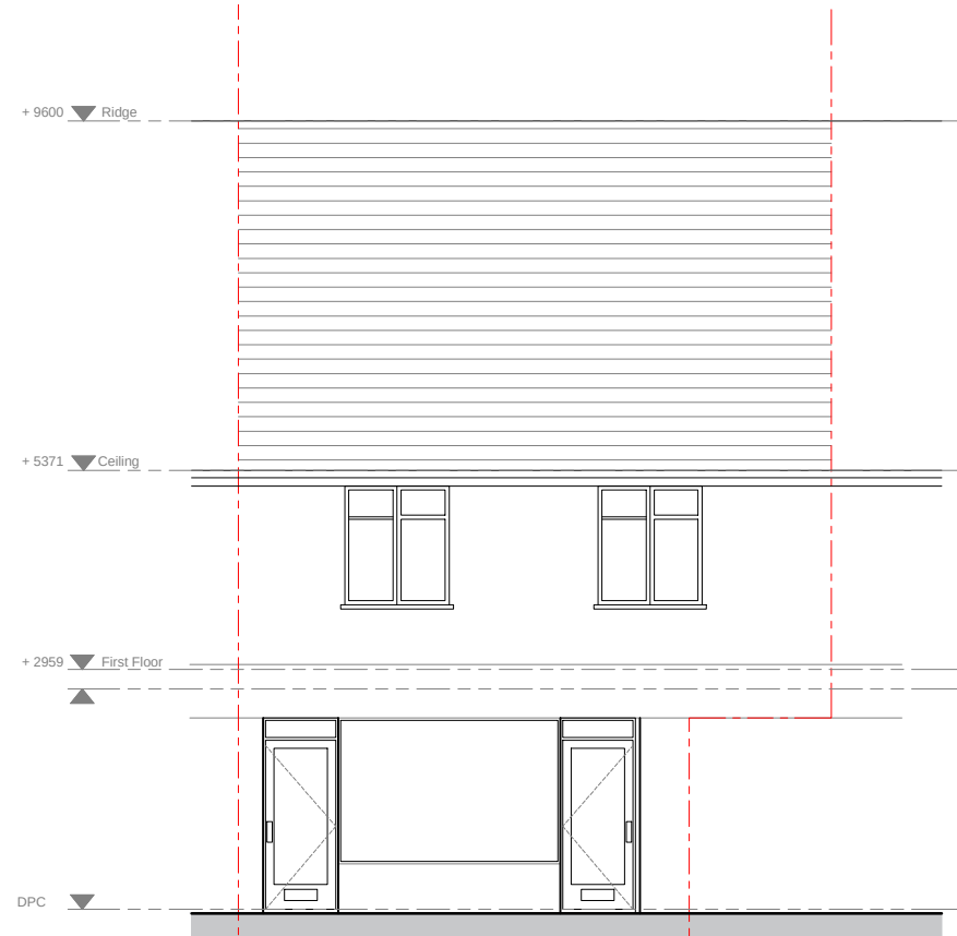
Front Elevation ( To the Winchester Road)
