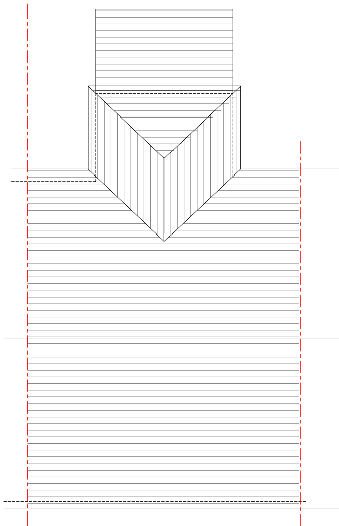
Roof Plan
