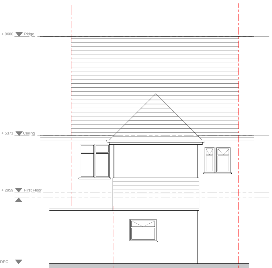
Rear Elevation
