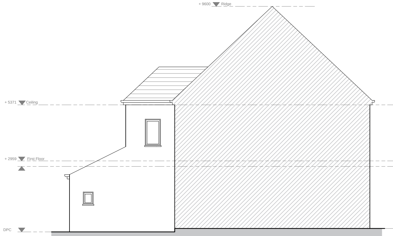
Side Elevation 1
