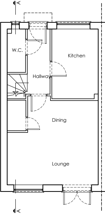
Existing Ground Floor Plan Scale 1/100@A3
