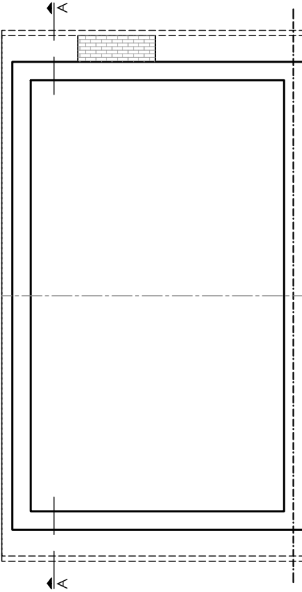
Existing Loft Plan Scale 1/100@A3
