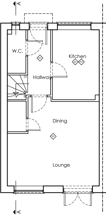
Proposed Ground Floor Plan Scale 1/100@A3
