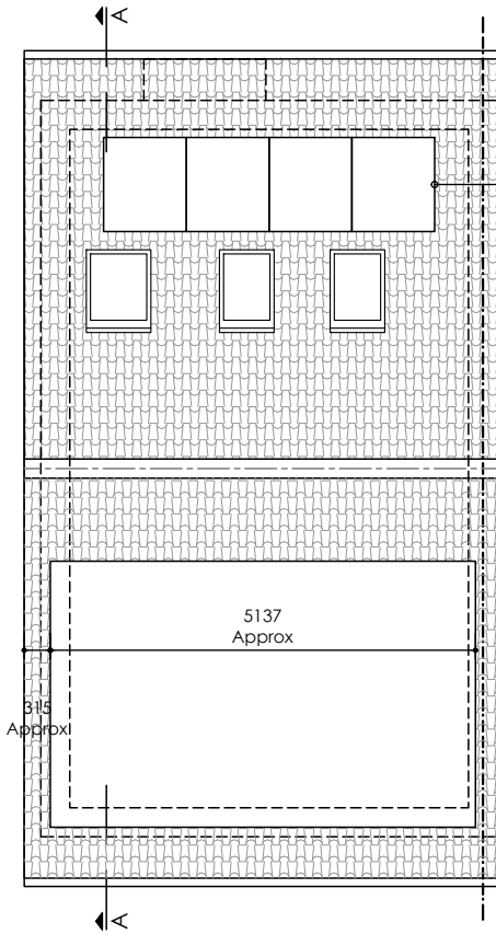
Proposed Roof Plan Scale 1/100@A3
